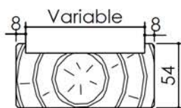
Traverse
