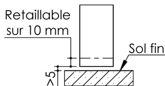
Sans joint balai
